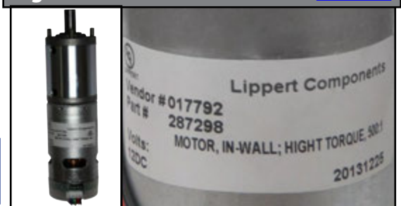
Fig. 4 - 500:1 Round Gearbox #287298
