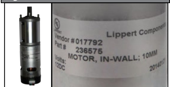
Fig. 3 - 300:1 Round Gearbox #236575
