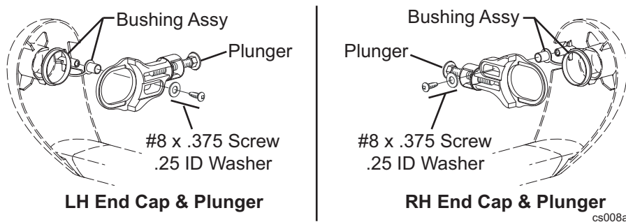
Figure 5. Plunger.
