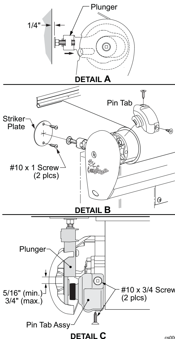
Figure 8. Anti-Billow Lock.
