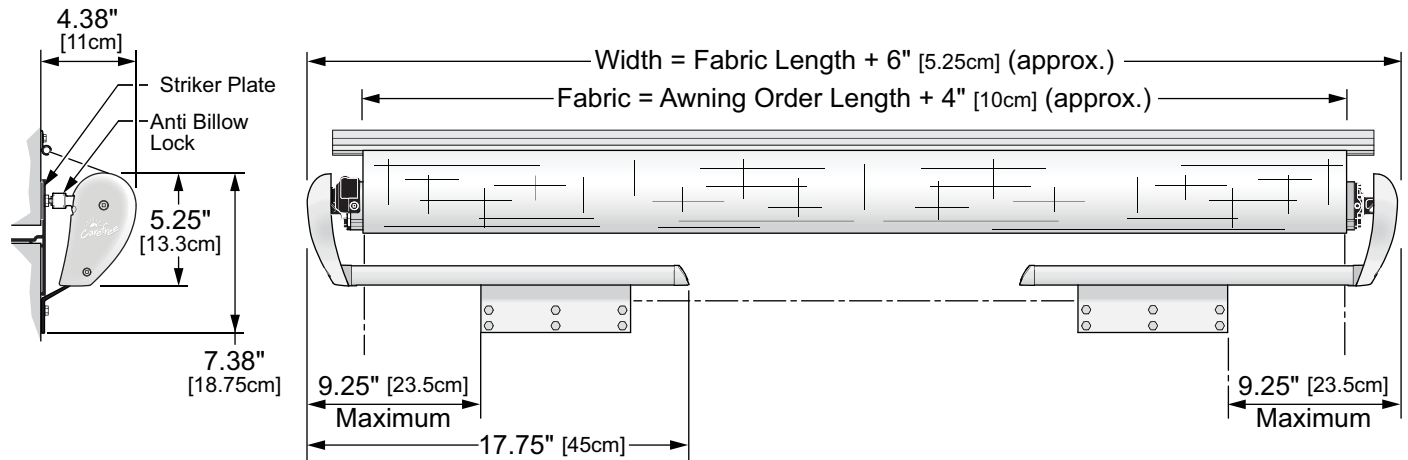
Figure 1. General Dimensions.
