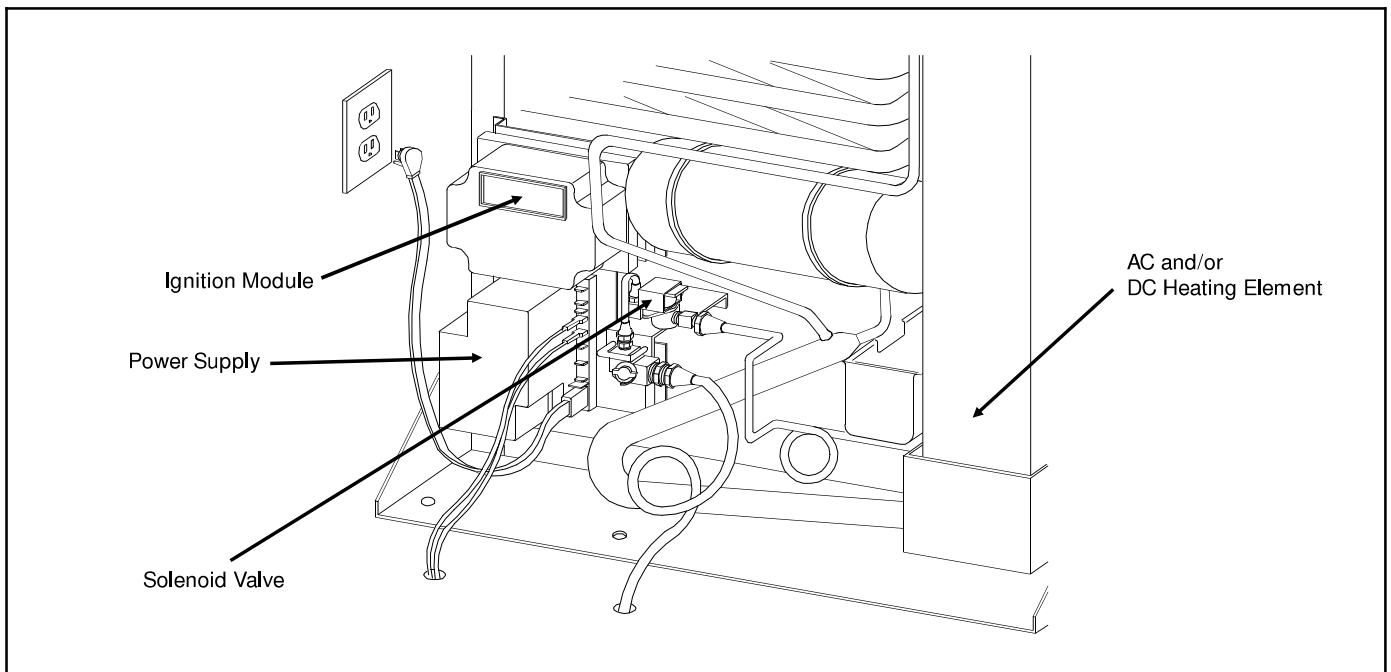
Figure 11.4 Rear View
