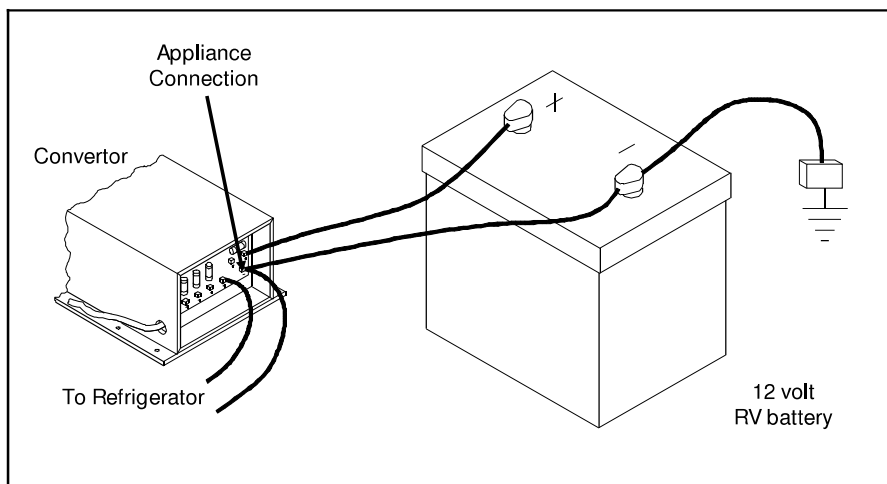
Figure 11.1 Recommended 12 Volt Supply Connection
