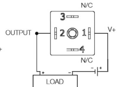
4-20mA OUTPUT
