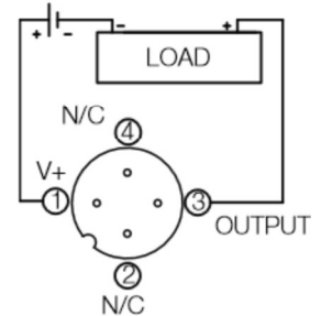
4-20mA OUTPUT
